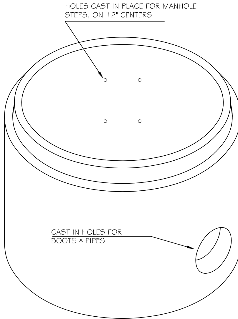
ISOMETRIC VIEW
