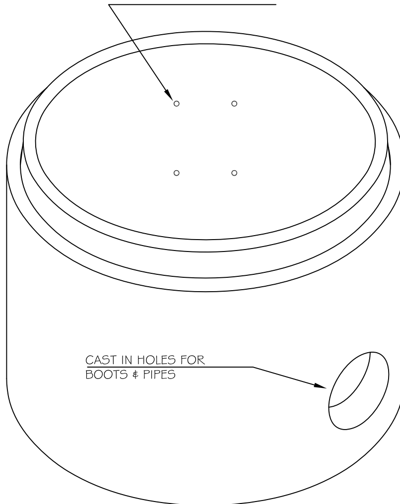
ISOMETRIC VIEW
